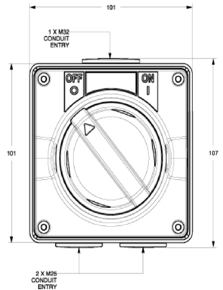
FRONT COMPLETE
