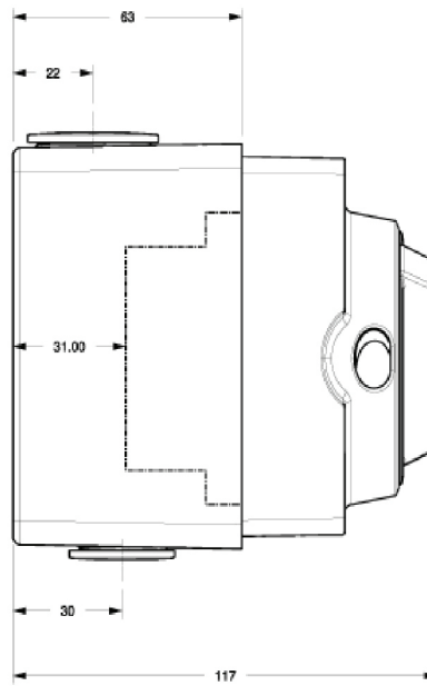
SIDE COMPLETE
