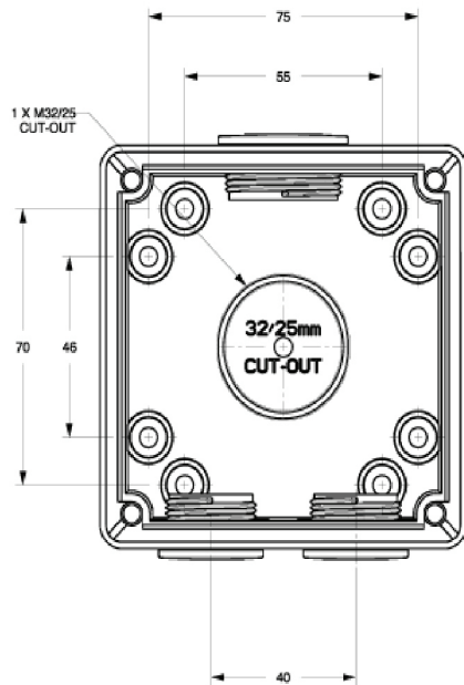
FRONT MOUNTING ENCLOSURE
