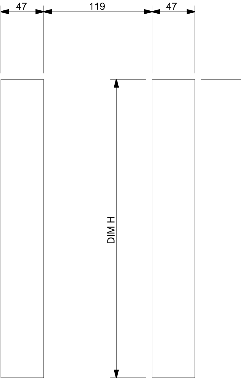
ESCUTCHEON CUTOUTS
