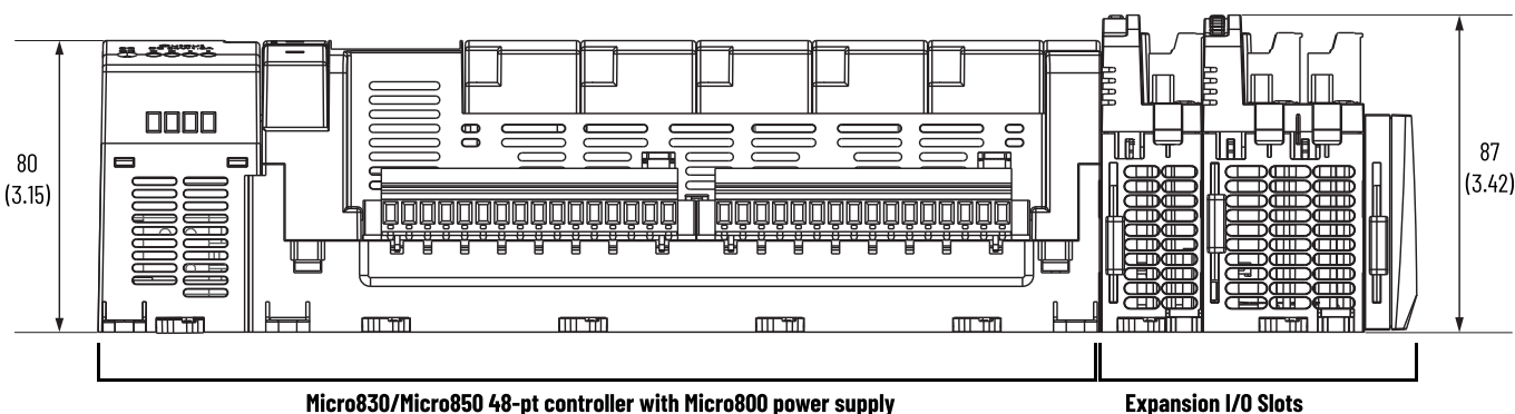
Micro830 and Micro850 48-point Controllers (Side)
