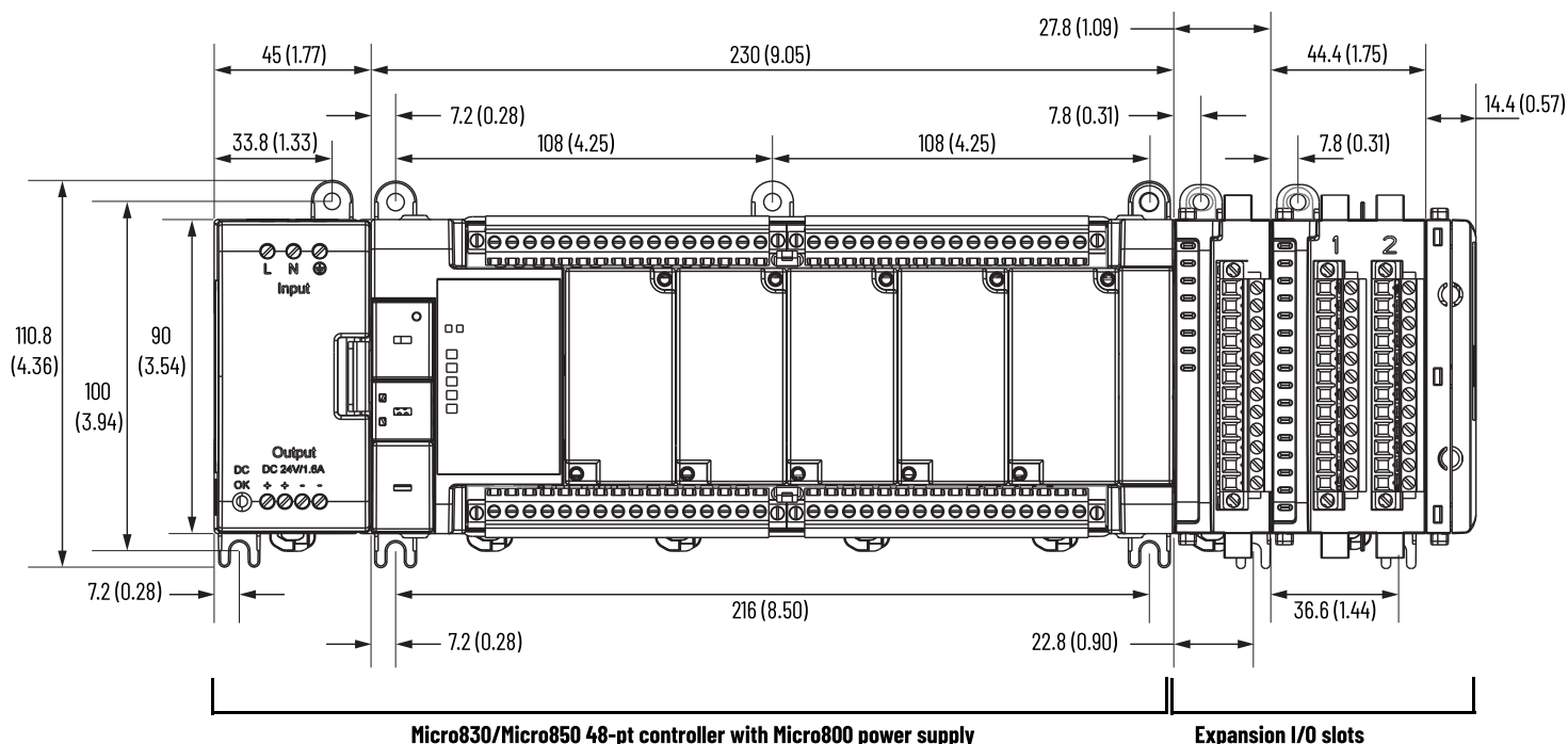
Micro830 and Micro850 48-point Controllers (Front)
