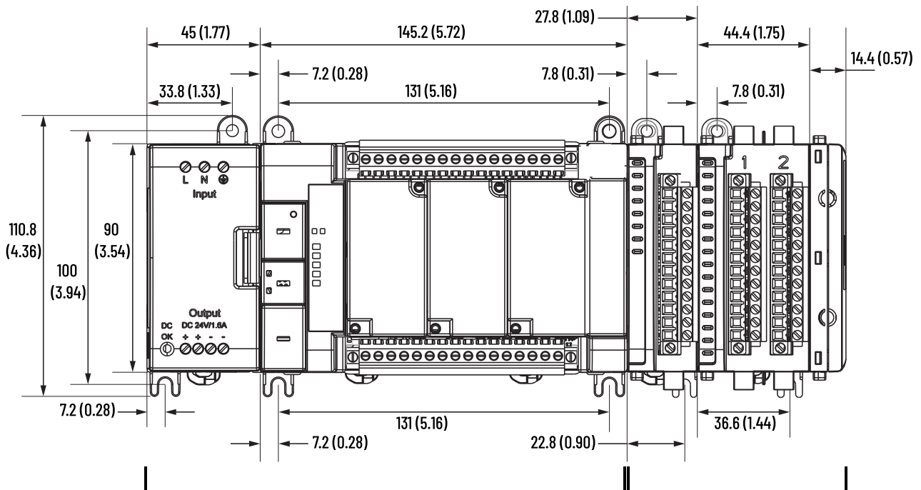
Micro830, Micro850, and Micro870 24-point Controllers (Front)
