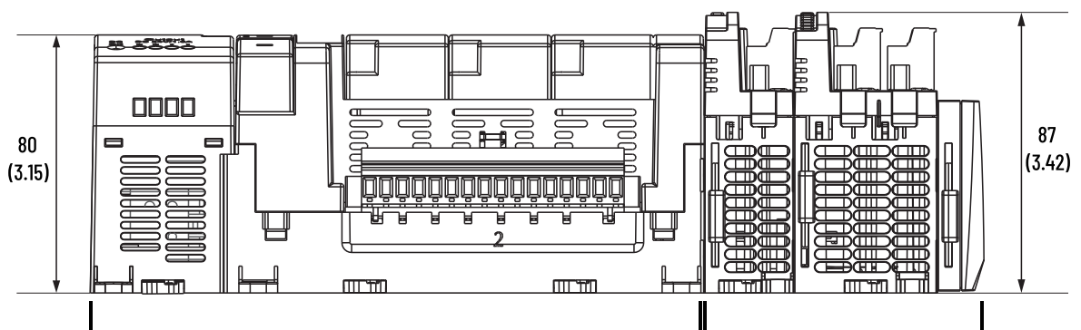
Micro830, Micro850, and Micro870 24-point Controllers (Side)
