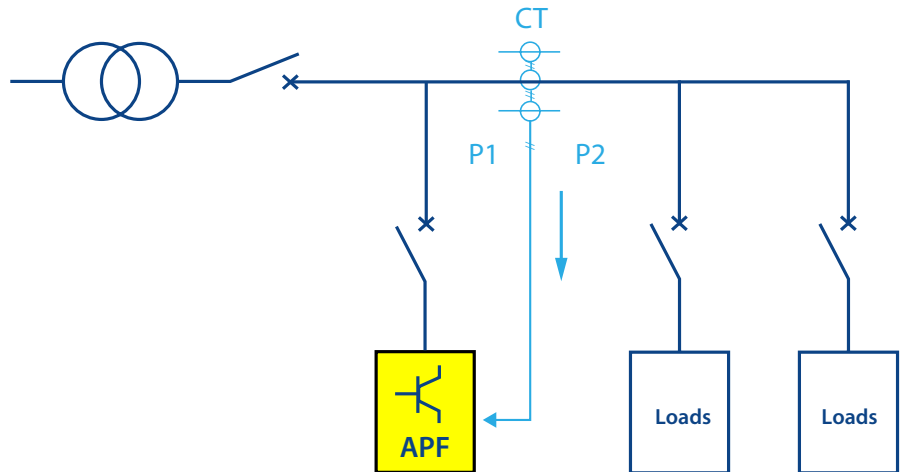
Figure 2-1 CT Connection for open loop, without cap bank scenario – SLD
