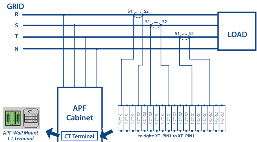
Figure 2-2 CT Connection for open loop, without cap bank scenario – Detailed
